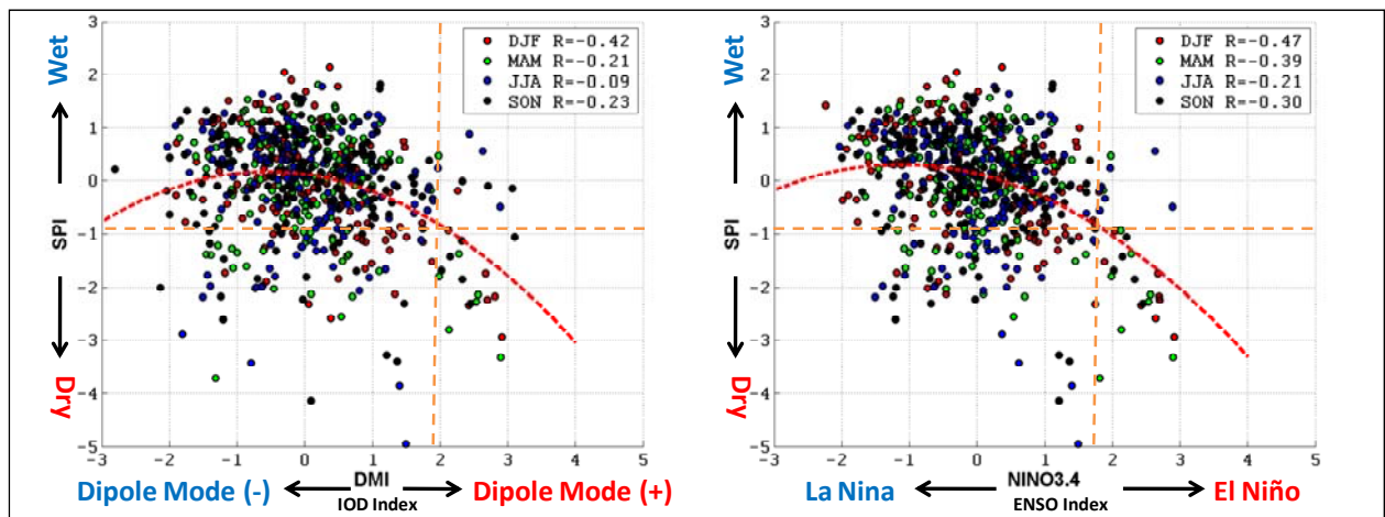
Figure 2.3 Correlation between 6-monthly Standardized Precipitation Index (SPI) calculated from rainfall of Tarakan and Dipole Mode Index (DMI)(left) as well as ENSO index (Nino3.4 sea surface anomaly)(right).
